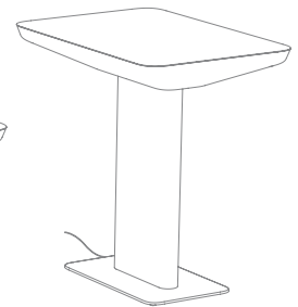
105 | 700 x 1000 x H1050
